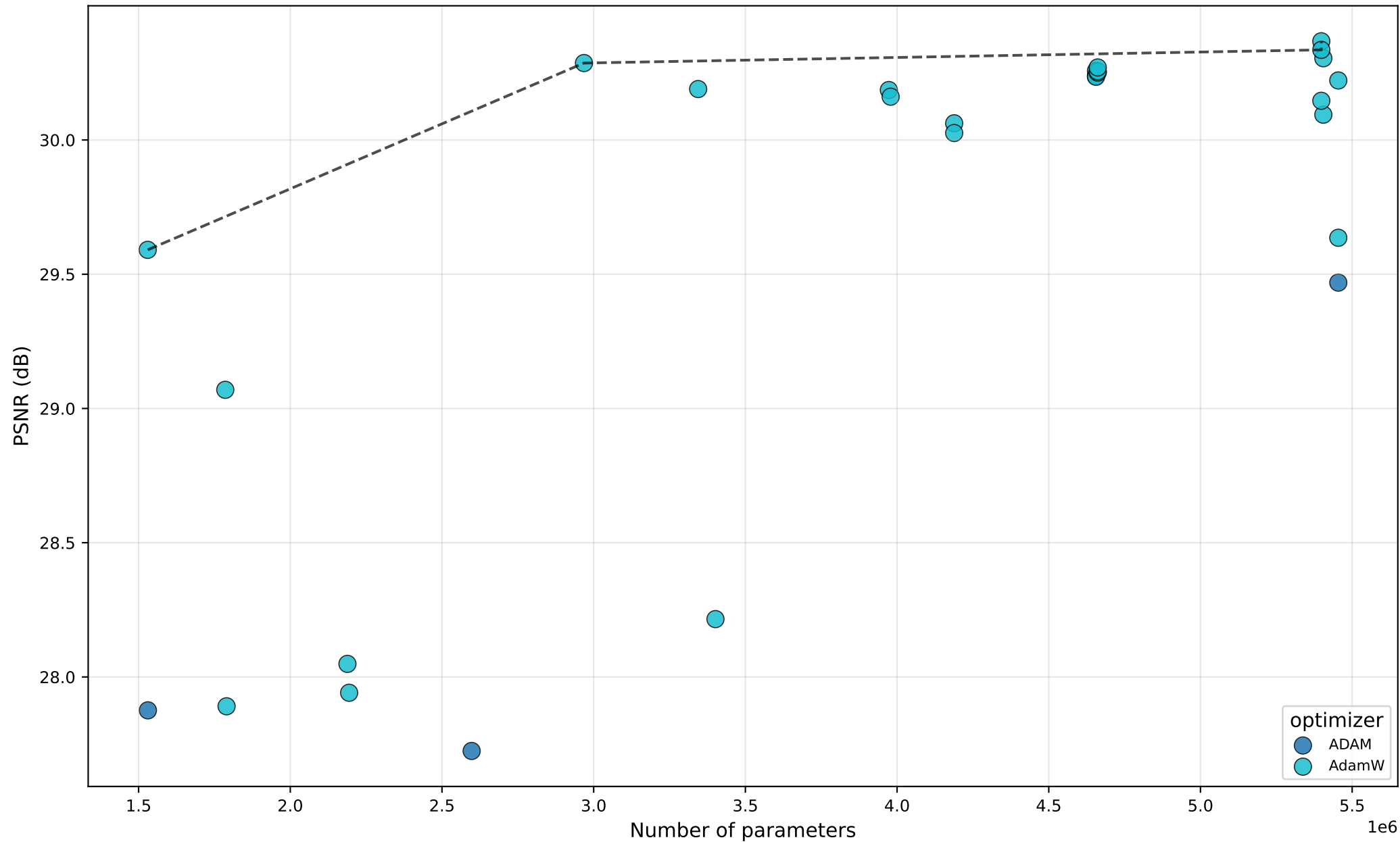
PSNR vs #Params — WaveletAttention — by optimizer
